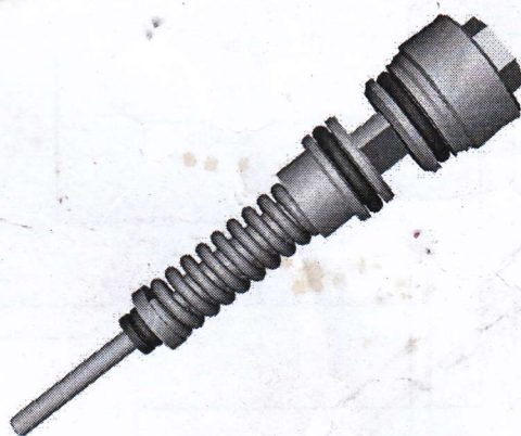
Fig. 2: New control piston, without cylinder lining
