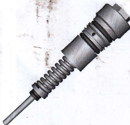
Fig. 1: Old control piston, with cylinder lining
